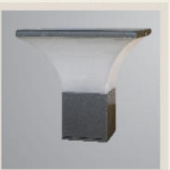
Kepler-Square
